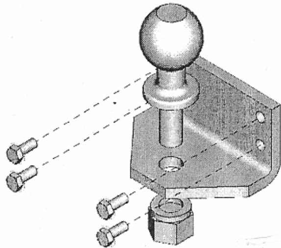
2 5/16" Ball Hitch
