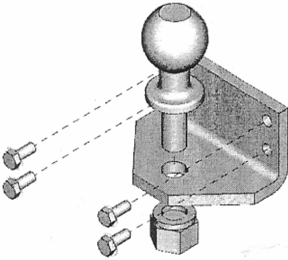
2" Ball Hitch
